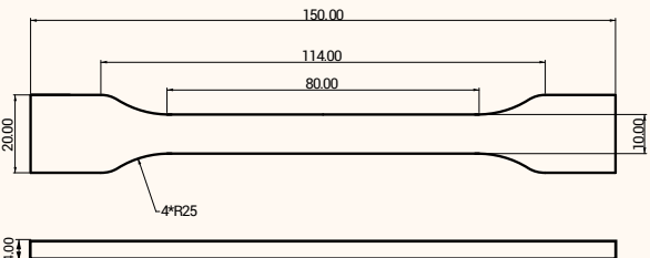
TENSILE TESTING SPECIMEN ISO 527
